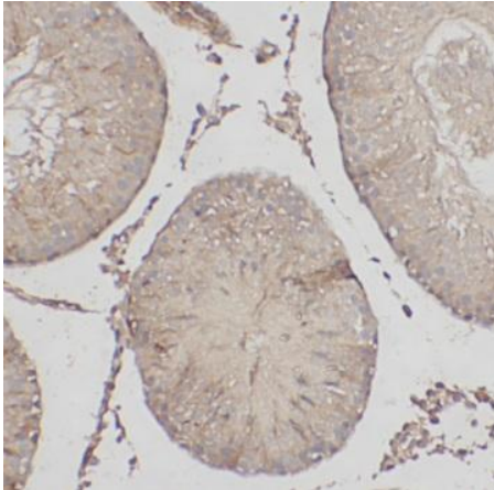
Immunohistochemistry of paraffin-embedded Rat testis tissue slide using FNab10210(LTOR1 antibody) at dilution of 1:200
